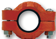
Standard Coupling 1,000 PSI #GVC-S
