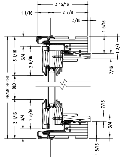
Vertical Section
