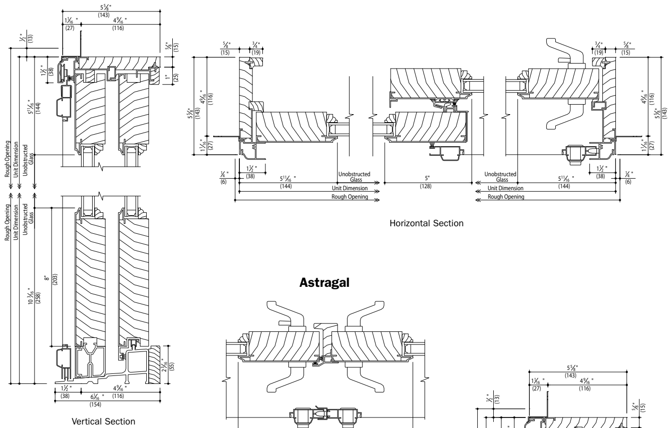
Vertical Section
