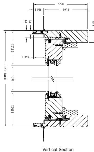
Vertical Section
