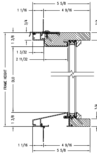
Vertical Section
