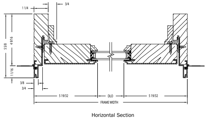
Horizontal Section
