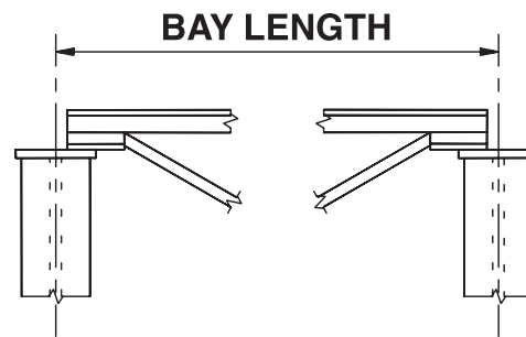
STEEL COLUMN
