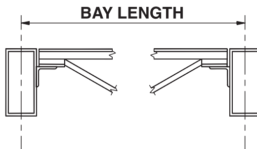
STEEL TUBE
