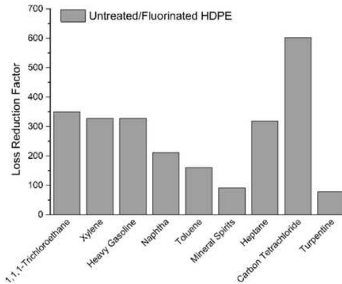
FIGURE 2 RATIO OF PRODUCT LOSS OF UNTREATED AND FLUORINATED HDPE IN A 125ML CONTAINER WITH 1MM WALL THICKNESS AT 50°C
