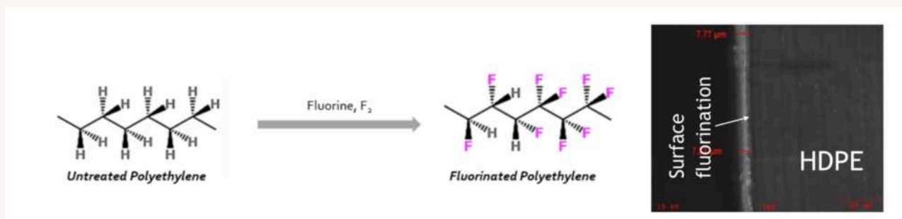
FIGURE 1 CHEMICAL MODIFICATION OF HDPE SURFACE AND SCANNING ELECTRON MICROGRAPH OF MODIFIED HDPE SURFACE.
