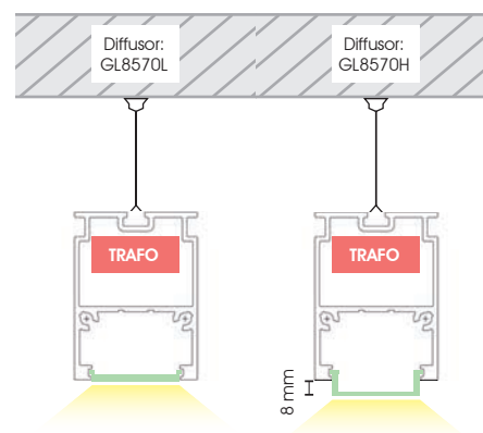
Pendelversion / pending
